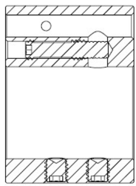
SECTION A-A Gas Blocked
